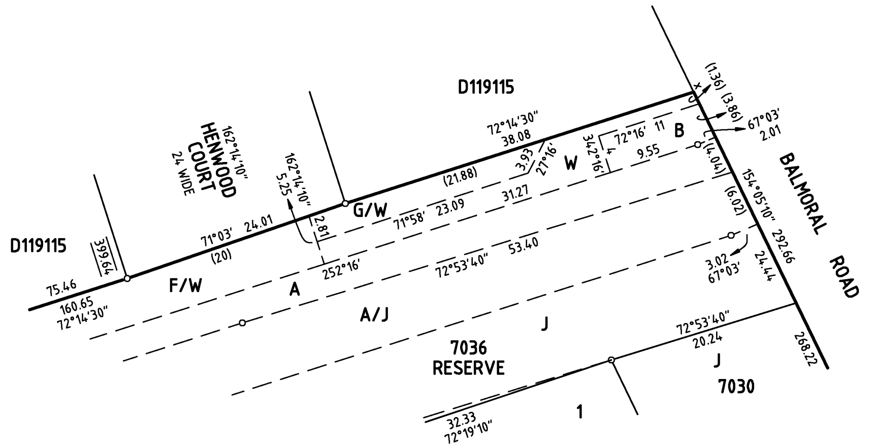
ENLARGEMENT A7 SCALE AS SHOWN
