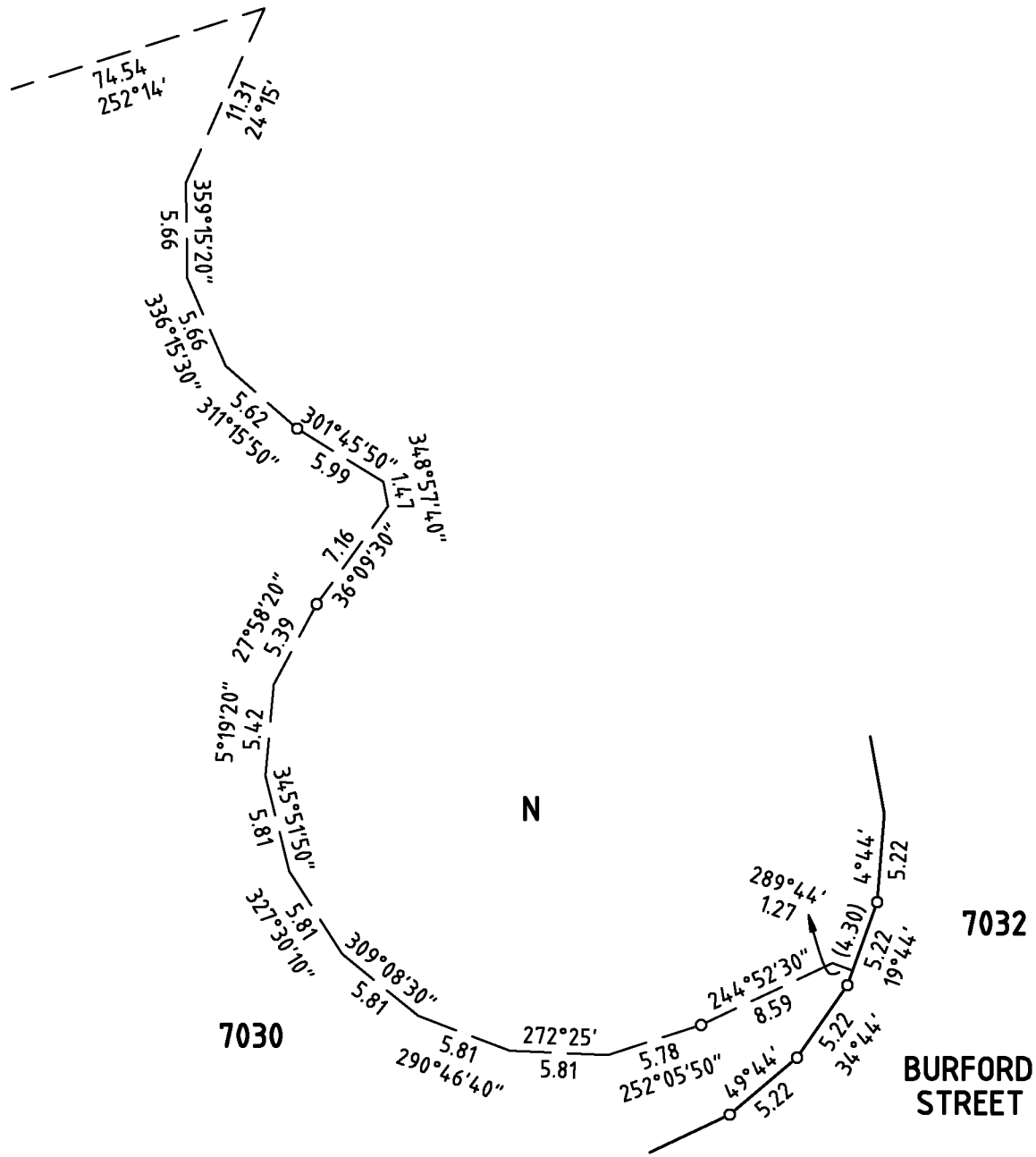
ENLARGEMENT B7 SCALE AS SHOWN
